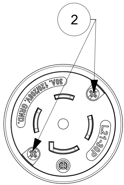
FACE VIEW
