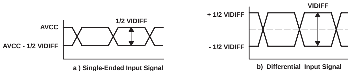
Figure 15. TMDS Inputs
