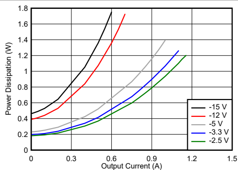
Figure 4-2. Power Dissipation
