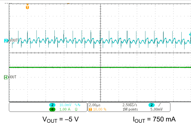
Figure 4-5. Output Ripple Waveform
