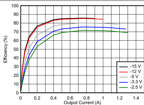
Figure 4-7. Efficiency
