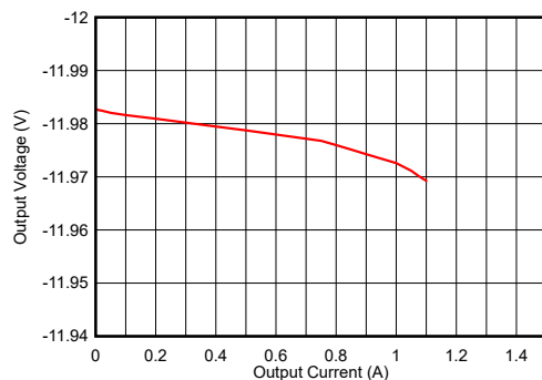
Figure 4-16. Load Regulation ( V_{OUT} = -12\text{ V} )
