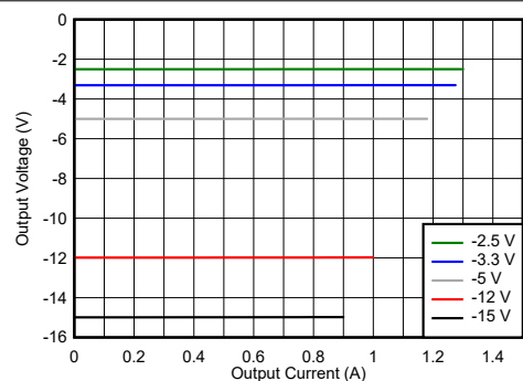
Figure 4-9. Load Regulation
