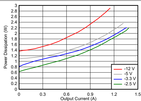
Figure 4-20. Power Dissipation
