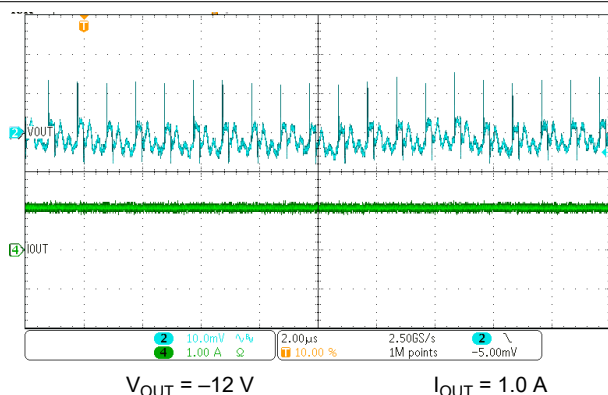
Figure 4-23. Output Ripple Waveform
