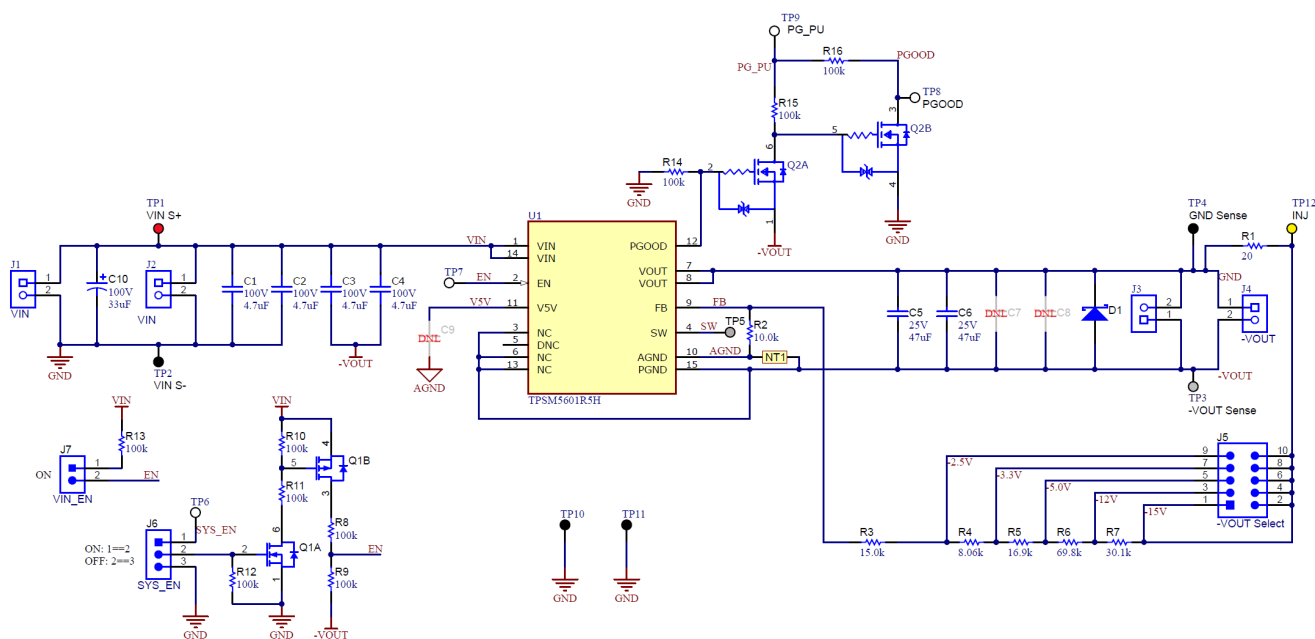
Figure 7-1. TPSM5601R5H-IBB-EVM Schematic
