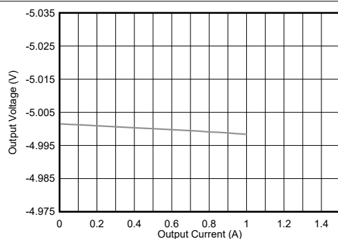
Figure 4-4. Load Regulation ( V_{OUT} = -5\text{ V} )
