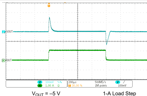
Figure 4-12. Transient Response Waveform
