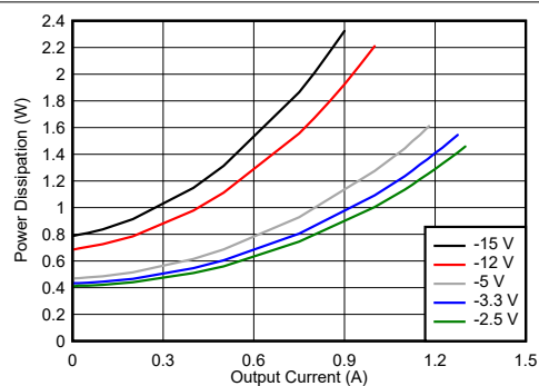
Figure 4-8. Power Dissipation
