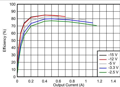
Figure 4-1. Efficiency
