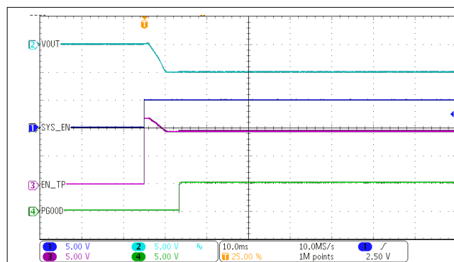
Figure 5-2. Enable Turn-On on V_{IN} = 24\text{ V}
