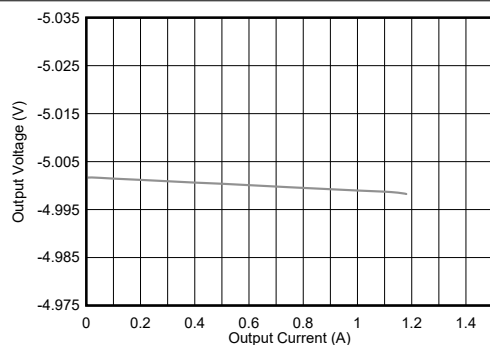
Figure 4-10. Load Regulation ( V_{OUT} = -5\text{ V} )
