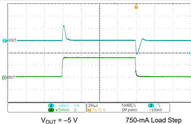
Figure 4-6. Transient Response Waveform
