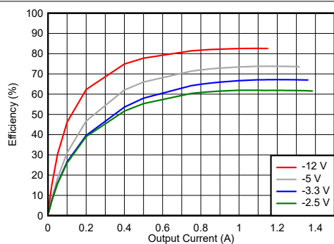
Figure 4-19. Efficiency
