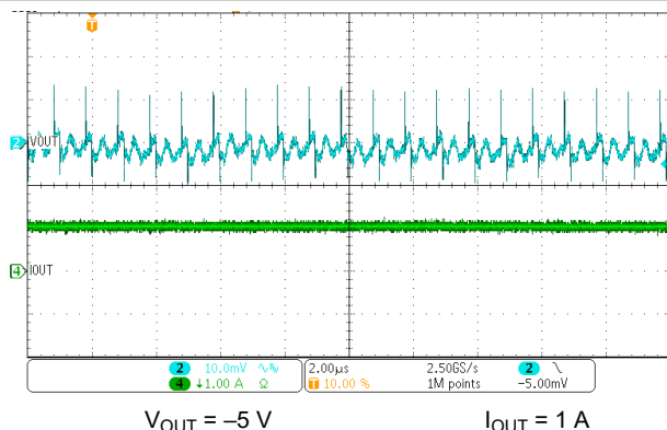
Figure 4-11. Output Ripple Waveform
