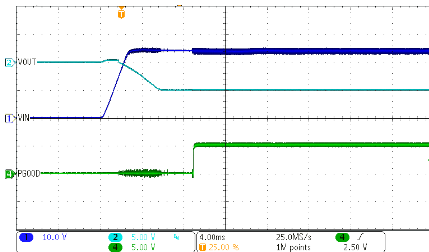
Figure 5-5. PGOOD Signal
