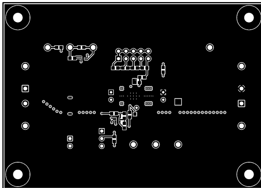
Figure 6-5. Bottom Layer
