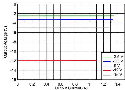
Figure 4-15. Load Regulation
