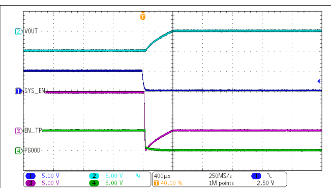
Figure 5-3. Enable Turn-Off on V_{IN} = 24\text{ V}
