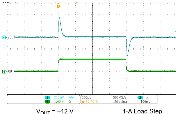
Figure 4-18. Transient Response Waveform
