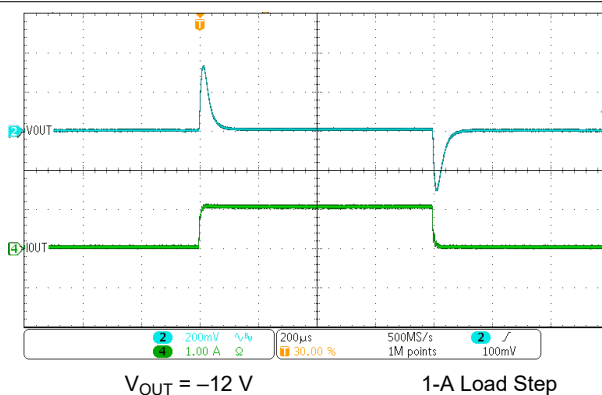
Figure 4-24. Transient Response Waveform
