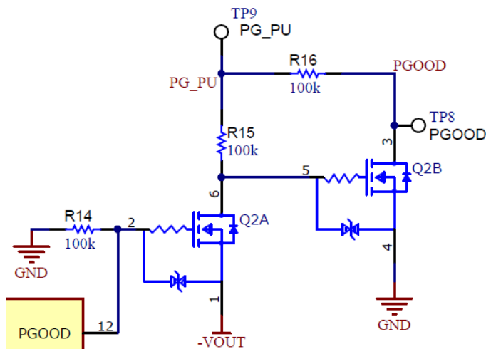
Figure 5-4. PGOOD Level-Shifter
