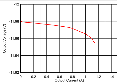
Figure 4-22. Load Regulation ( V_{OUT} = -12\text{ V} )
