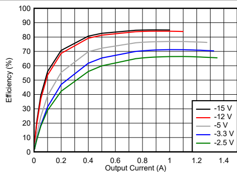
Figure 4-13. Efficiency
