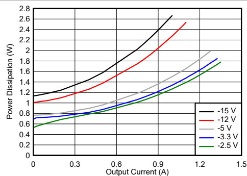
Figure 4-14. Power Dissipation
