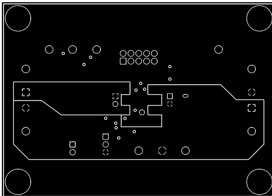
Figure 6-3. Signal Layer 1
