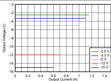
Figure 4-3. Load Regulation
