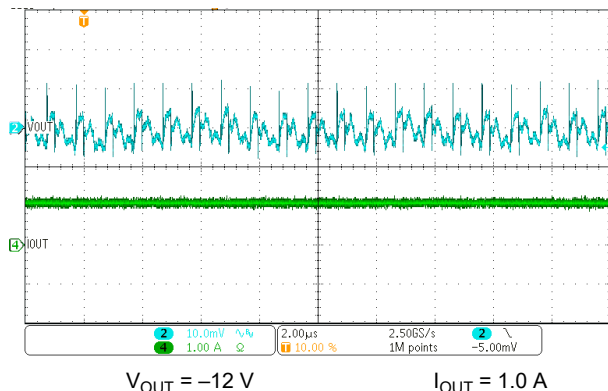
Figure 4-17. Output Ripple Waveform
