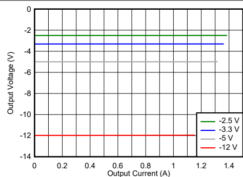
Figure 4-21. Load Regulation
