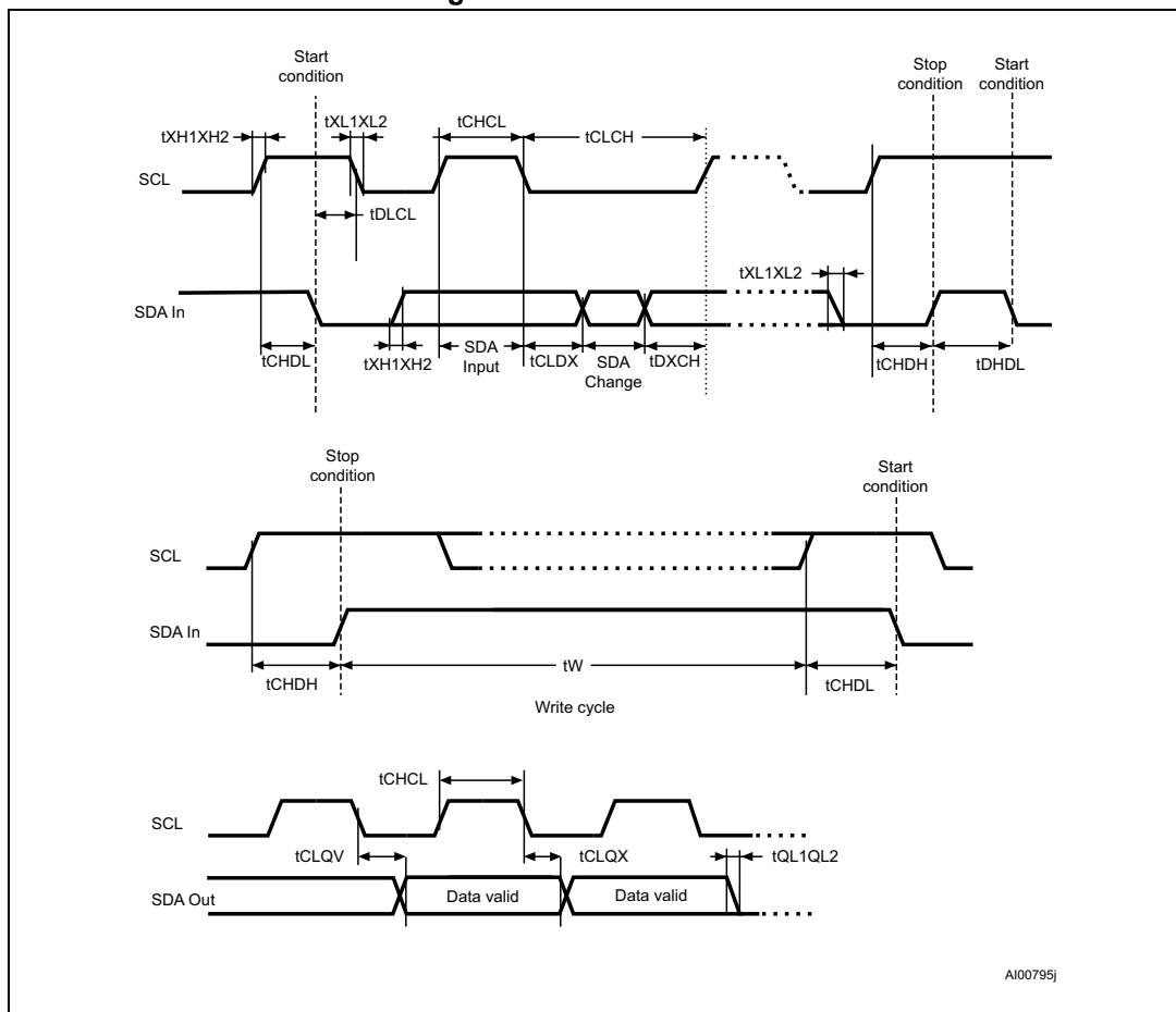
Figure 10. AC waveforms
