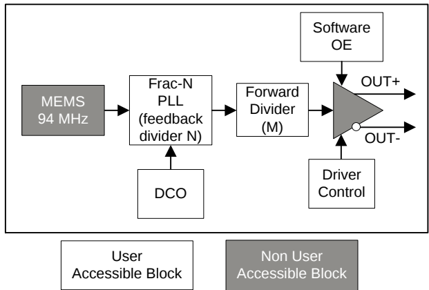
Figure 25. In-system Programmable Oscillator Block Diagram
