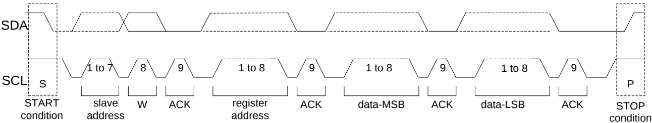
Figure 35. Write Sequence
