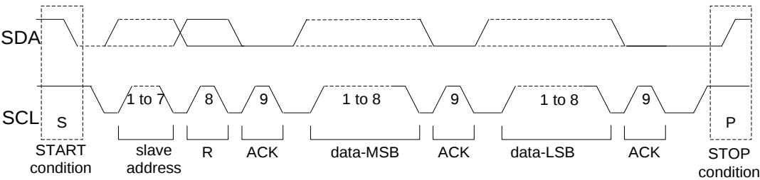
Figure 36. Read Sequence
