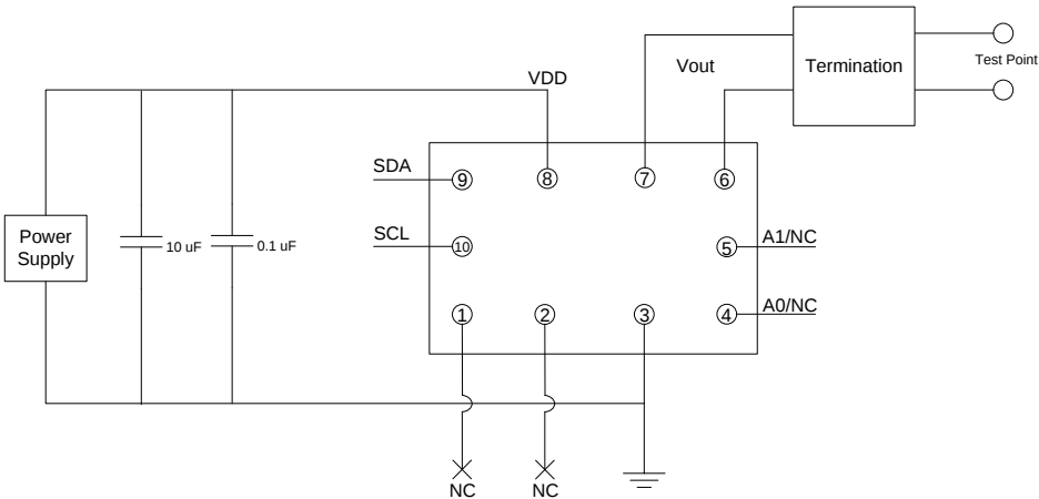
Figure 21. Test Circuit (I²C mode and NC Function for both Pin1 and Pin2)
