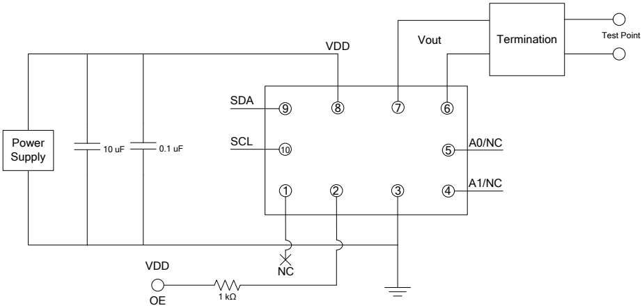
Figure 20. Test Circuit (I²C mode and OE Function for Pin 2)
