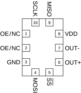
Figure 4. SPI Mode
