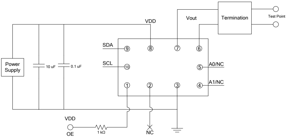
Figure 19. Test Circuit (I²C mode and OE Function for Pin 1)
