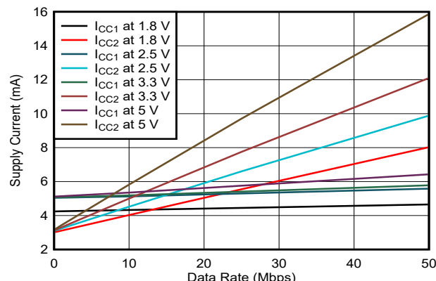
Figure 7-3. ISO6760 Supply Current vs Data Rate (With 15-pF Load)
