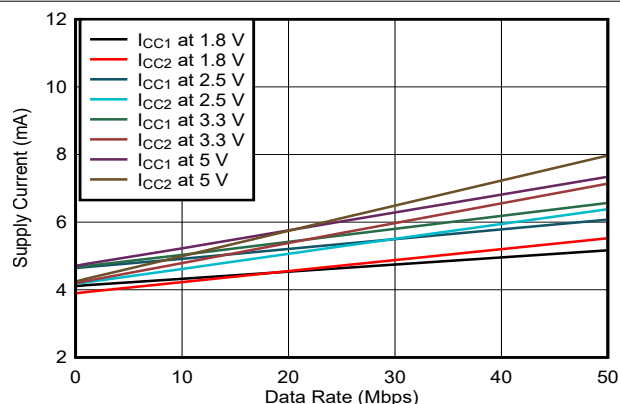
Figure 7-6. ISO6761 Supply Current vs Data Rate (With No Load)
