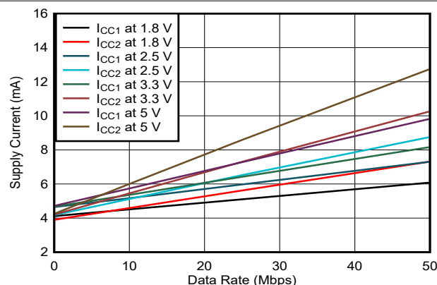
Figure 7-5. ISO6761 Supply Current vs Data Rate (With 15-pF Load)
