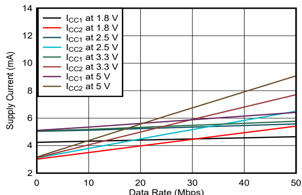
Figure 7-4. ISO6760 Supply Current vs Data Rate (With No Load)
