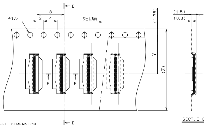
REEL DIMENSION
