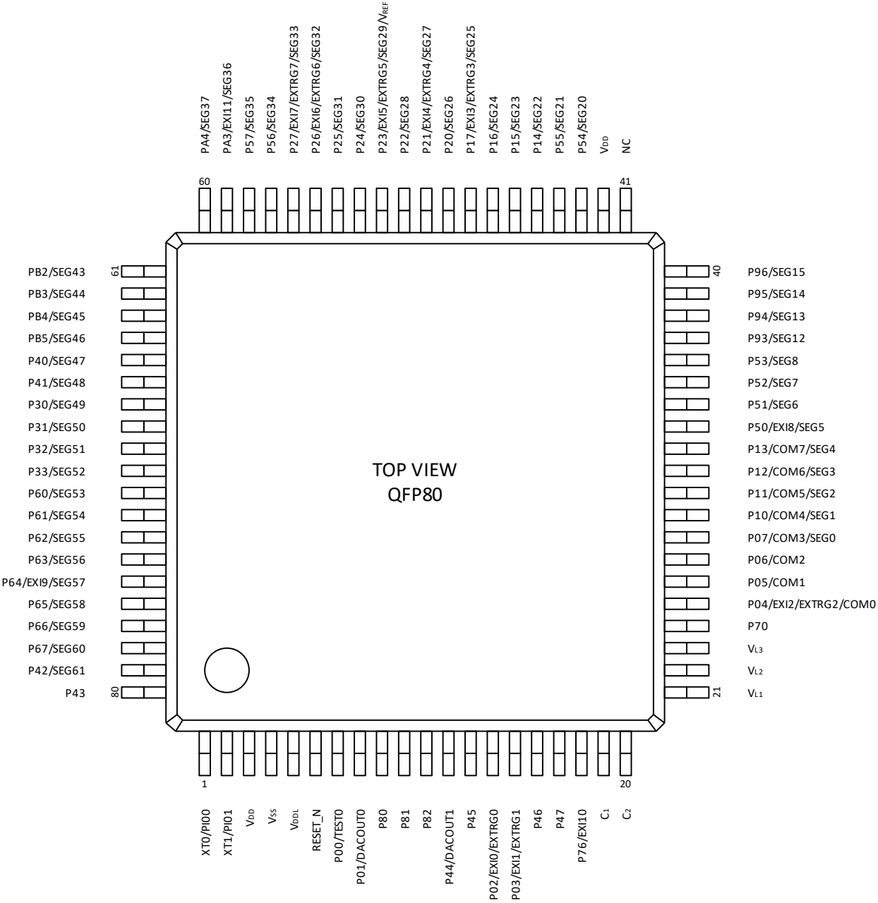
Figure 6 Pin Layout of 80pin QFP Package
