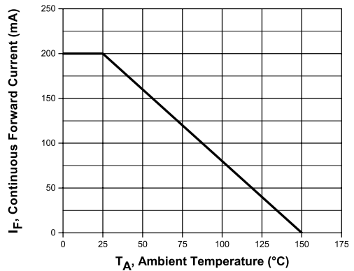
Current Derating
