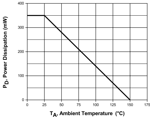
Power Derating
