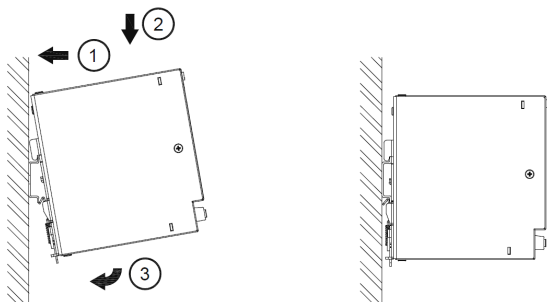
Fig. 2.1 Mounting
