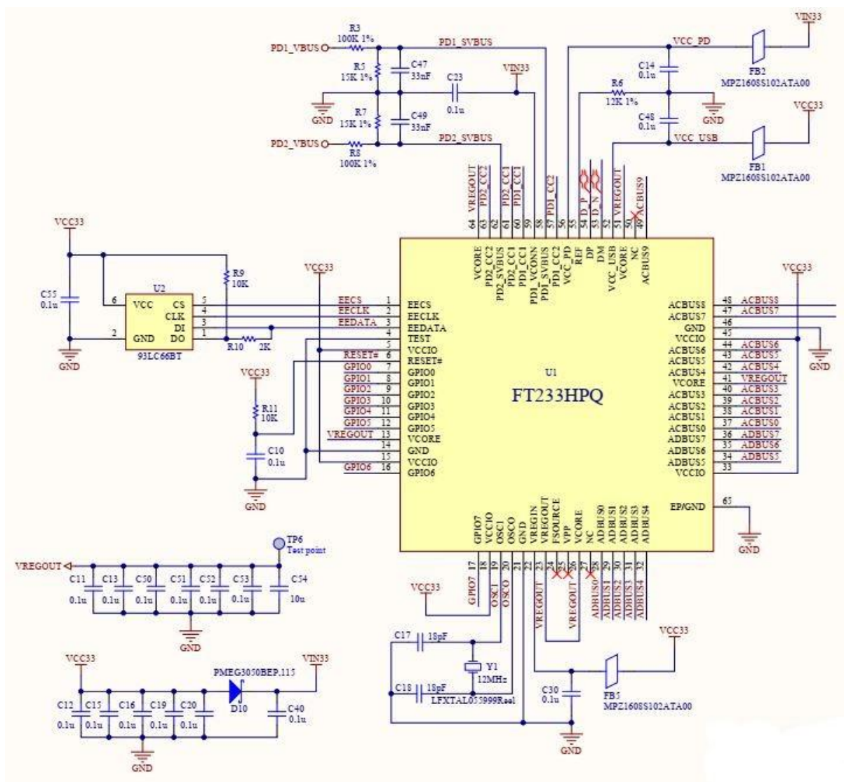
Figure 5 – FT233HPQ IC
