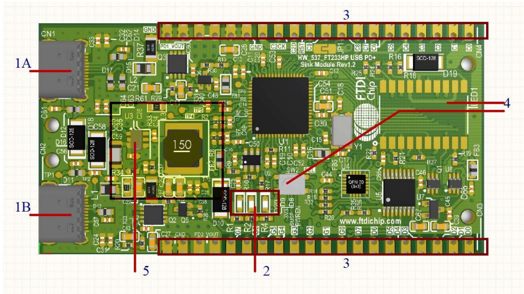
Figure 2 - UMFT233HPEV-SD Sink Module Board - Top View
