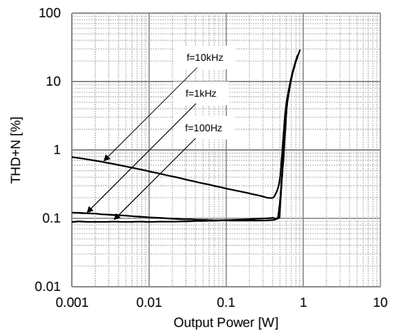
THD+N vs. Output Power [Differential Input] V^+=5V, R_L=16\Omega BW: 22-22kHz( f=100\text{Hz} , 1kHz), 22-80kHz( f=10\text{kHz} )
