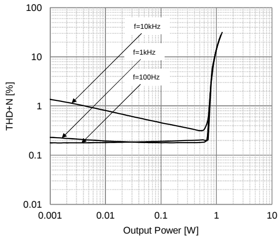
THD+N vs. Output Power [Differential Input] V^+=5V, R_L=8\Omega BW: 22-22kHz( f=100\text{Hz} , 1kHz), 22-80kHz( f=10\text{kHz} )
