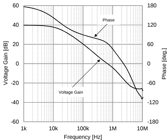
Voltage Gain / Phase vs. Frequency V^+=5V , R_L=16\Omega , G_v=40dB
