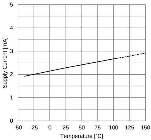
Supply Current vs. Temperature V^+ = +3.3\text{V} , R_L = \text{Open} , No signal
