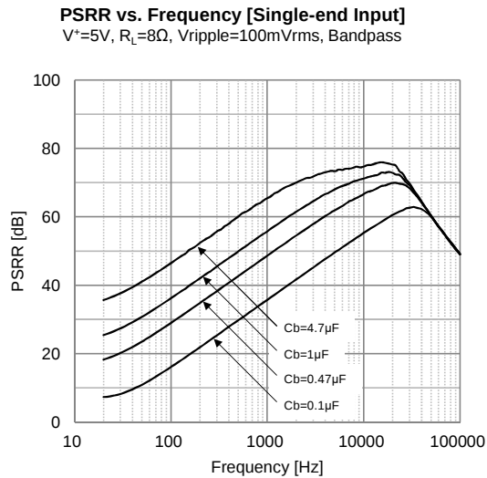
Fig. 12 PSRR vs. C_b (Single-end input, V^+=5V )
