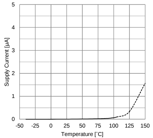
Supply Current vs. Temperature [Shutdown] V^+ = +3.3\text{V} , R_L = \text{Open} , No signal
