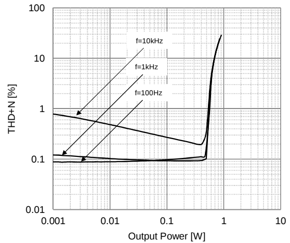
THD+N vs. Output Power [Differential Input] V^+=5V, R_L=16\Omega BW: 22-22kHz( f=100\text{Hz} , 1kHz), 22-80kHz( f=10\text{kHz} )
