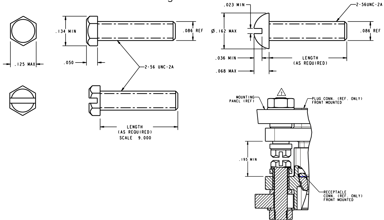
Float Mounting
