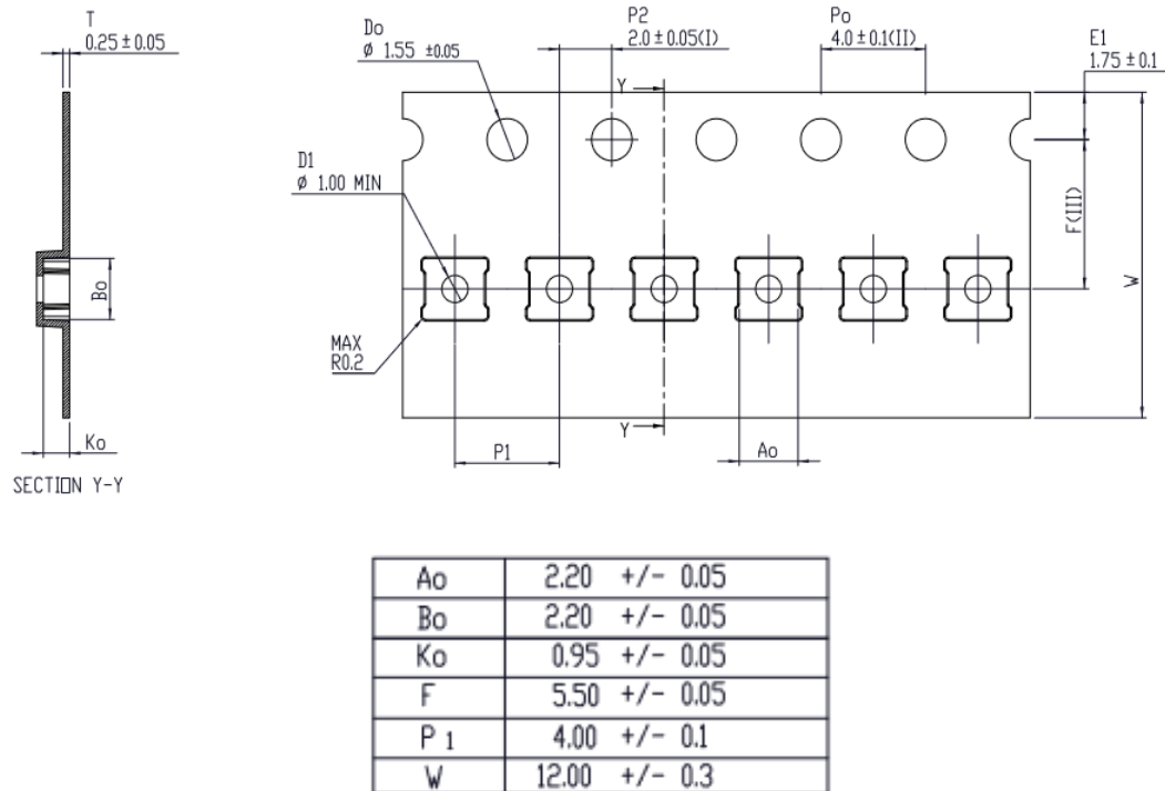
Figure 28: Tape and Reel dimensions
