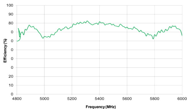
5 GHz Efficiency
