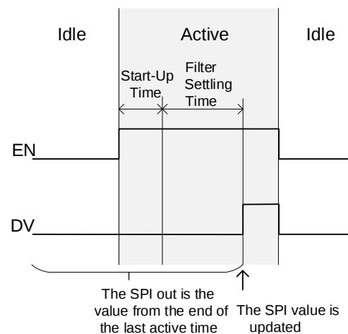
Figure 30: Signal Timing for External Control
