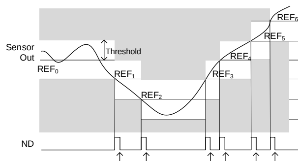
Figure 38: Example of the ND Signal when the Angle Changes (RAR = 1)
