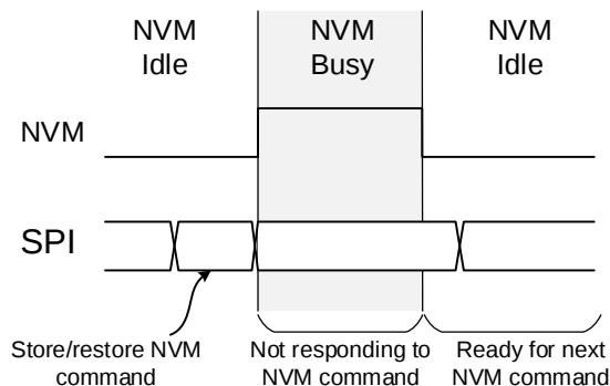
Figure 17: Signal Timing for NVM Access
