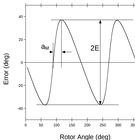
Figure 25: Error Curve in Side-Shaft Configuration (BCT = 0)
