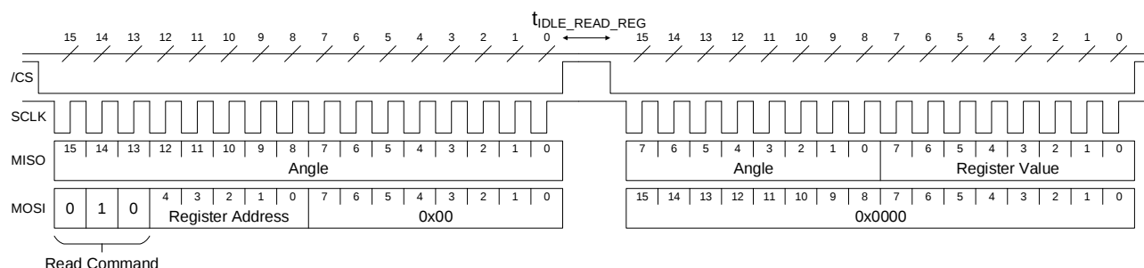
Figure 15: Two 16-Bit Frames Read Register Operation
