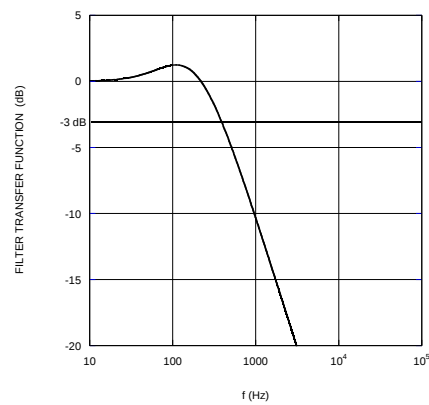
Filter Transfer Function FW = 10
