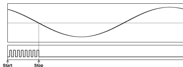
Top: Sine Waveform Bottom: Clock for Time-to-Digital Converter Figure 2: Phase Detection Method
