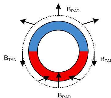
Figure 23: Side-Shaft Field
