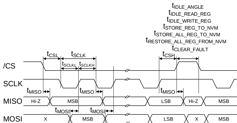
Figure 11: SPI Timing Diagram (Mode 3)
