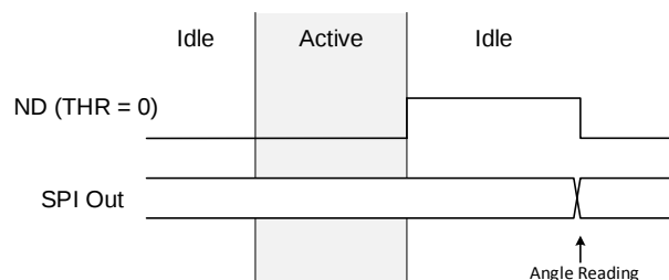
Figure 34: Using the ND Pin in Latch Mode as a Flag for Data Updates ( NDM = 0 , THR = 0 )
