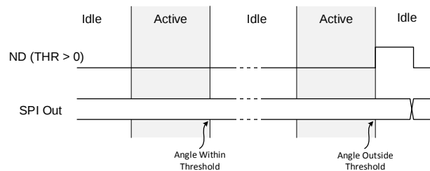
Figure 36: ND Pin Used at WOC Signal with a Non-Zero Threshold Setting (Latch Mode)
