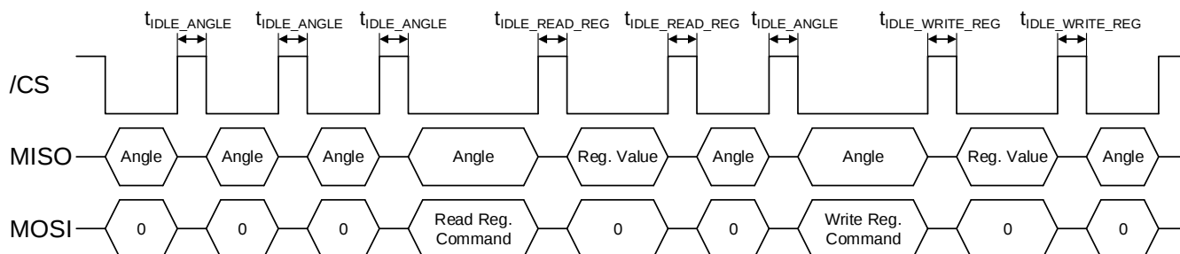
Figure 12: Minimum Idle Time
