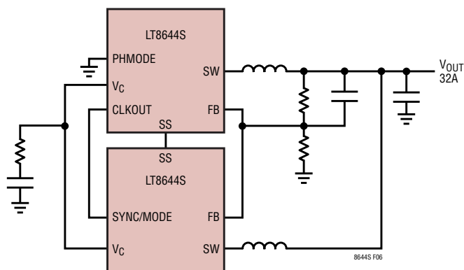
Figure 6. Paralleling Two LT8644Ss
