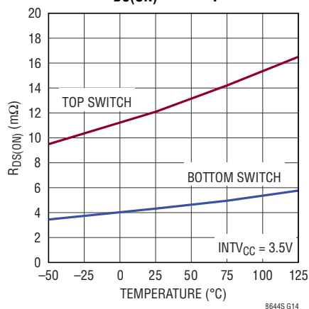
Switch R_{\text{DS(ON)}} vs Temperature
