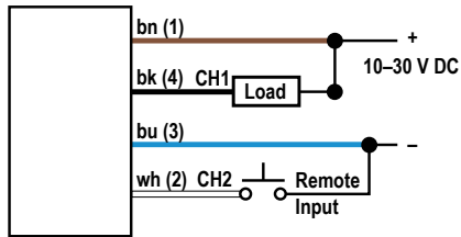
Figure 15. Channel 1 = NPN Output, Channel 2 = NPN Remote Input
