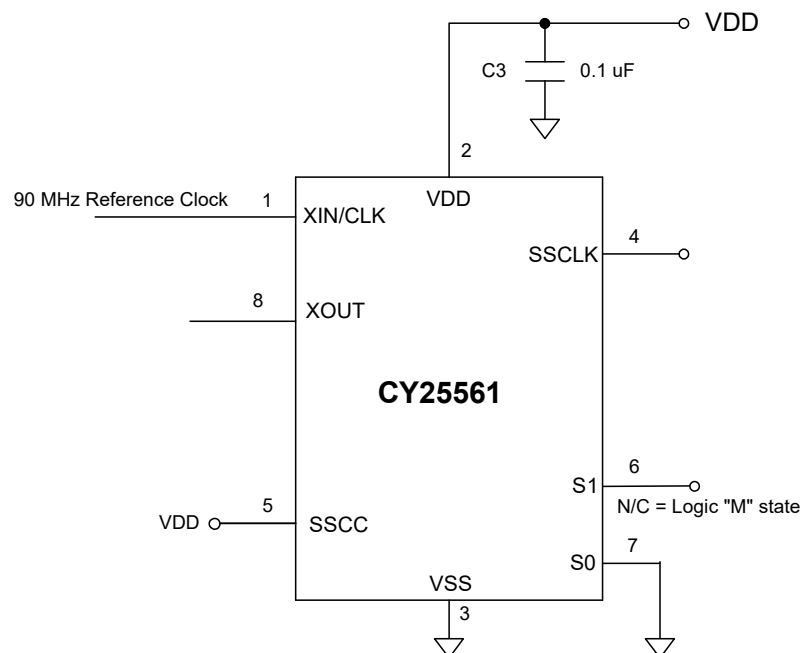
Figure 4. Application Schematic
