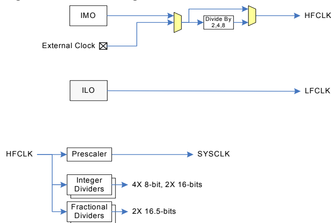
Figure 3. MCU Clocking Architecture
