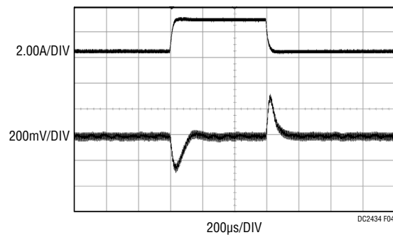
Figure 4. Transient Response Waveform at 14V IN and 2.5A–5A–2.5A OUT (2A, 200mV, 200μs/Div)
