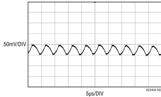
Figure 3. Output Ripple at 28V IN and 5A OUT (50mV, 5μs/Div, 20MHz)
