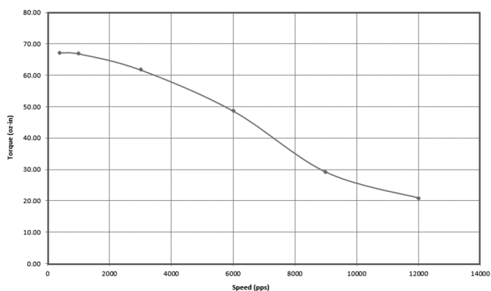
CUI Devices P/N NEMA23-17-01SD-AMT112S Lin Engineering P/N WO-5718X-01S (1.8 Step Motor) 24 Vdc, 1.4 Amp/Phase, Bipolar, 1/2 Stepping
