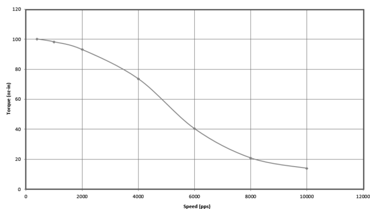
CUI Devices P/N NEMA23-17-01PD-AMT112S Lin Engineering P/N WO-5718X-01P (1.8 Step Motor) 24 Vdc, 2.8 Amp/Phase, IB463, 1/2 Stepping
