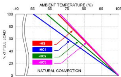
RED60-24S05W Derating Curve With Heat-sink
