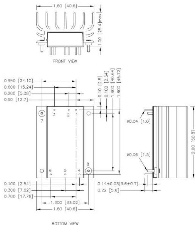
BOTTOM VIEW
