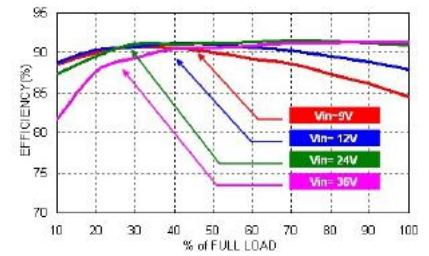
RED60-24S05W Efficiency vs. Output Load
