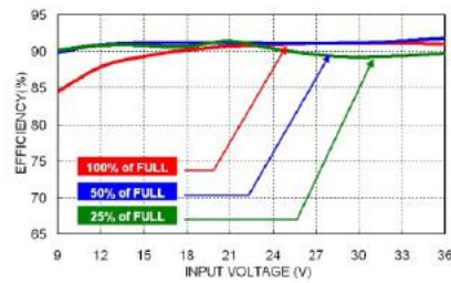
RED60-24S05W Efficiency vs. Input Voltage
