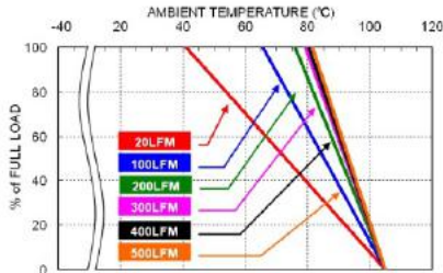
RED60-24S05W Derating Curve
