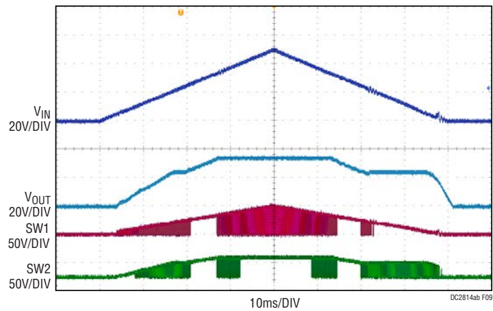
Figure 9. V_{IN} Range ( I_{OUT} = 2.5A )
