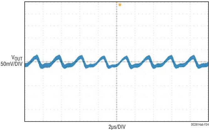
Figure 24. DC2814A-B Output Voltage Ripple at 40V IN (Buck), 34V OUT , 2.5A Load Current
