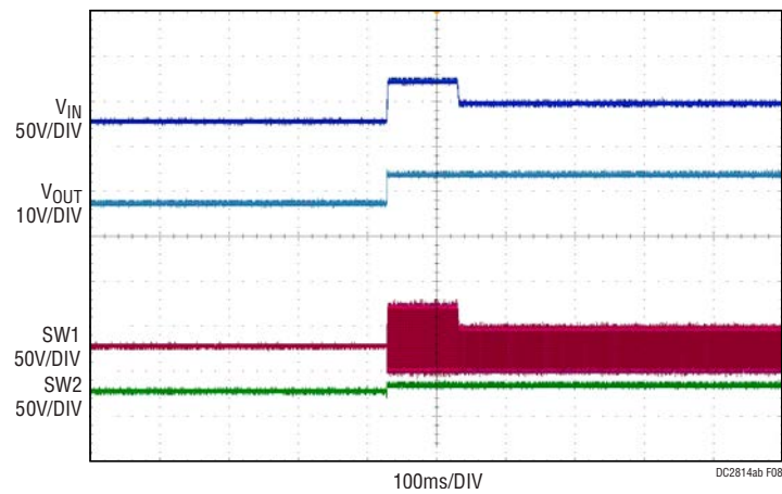
Figure 8. D0-160 – Abnormal Surge Voltage (Z) ( I_{OUT} = 2.5A )
