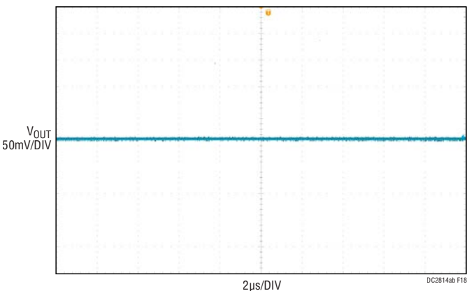
Figure 18. DC2814A-B Output Voltage Ripple at 30V IN (Pass-Thru), 30V OUT , 2.5A Load Current
