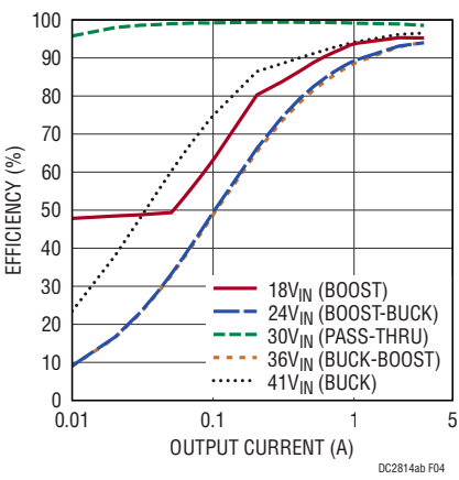
Figure 4. Efficiency vs Output Current
