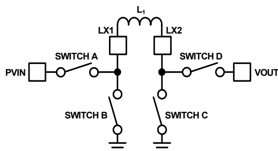
FIGURE 23. BUCK-BOOST TOPOLOGY
