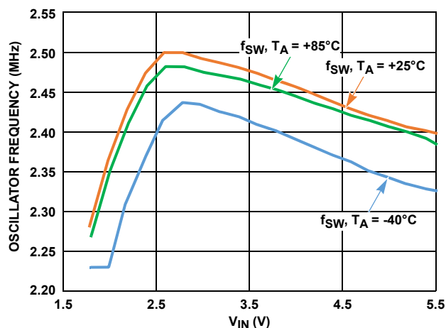
FIGURE 5. SWITCHING FREQUENCY vs INPUT VOLTAGE
