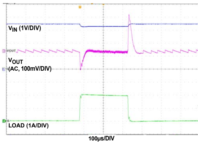
FIGURE 18. 0A TO 2A LOAD TRANSIENT, V_{IN} = 3.3\text{V}
