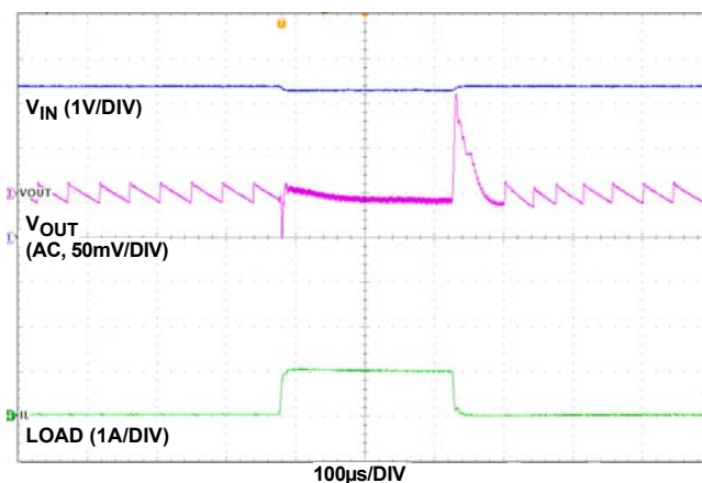
FIGURE 16. 0A TO 1A LOAD TRANSIENT, V_{IN} = 3.3\text{V}
