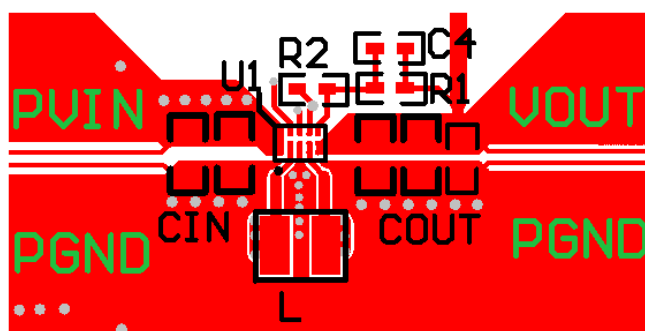
FIGURE 25. RECOMMENDED LAYOUT
