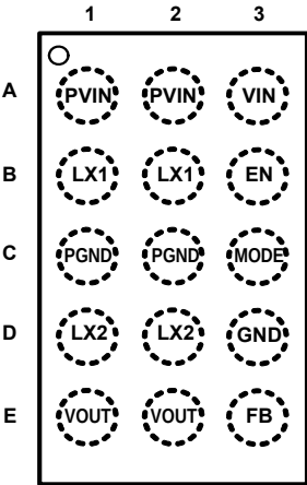
ISL91107 (15 BUMP WLCSP) TOP VIEW
