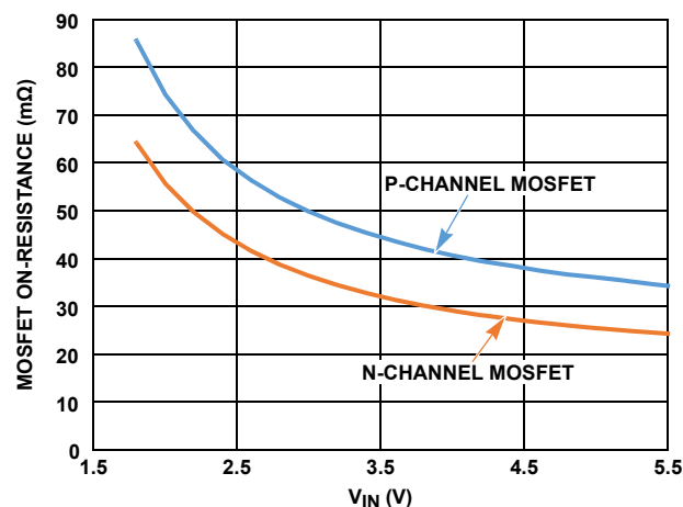
FIGURE 6. MOSFET ON-RESISTANCE vs INPUT VOLTAGE
