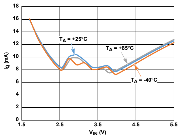
FIGURE 4. QUIESCENT CURRENT vs INPUT VOLTAGE (MODE = LOW, V_{OUT} = 3.3\text{V} )
