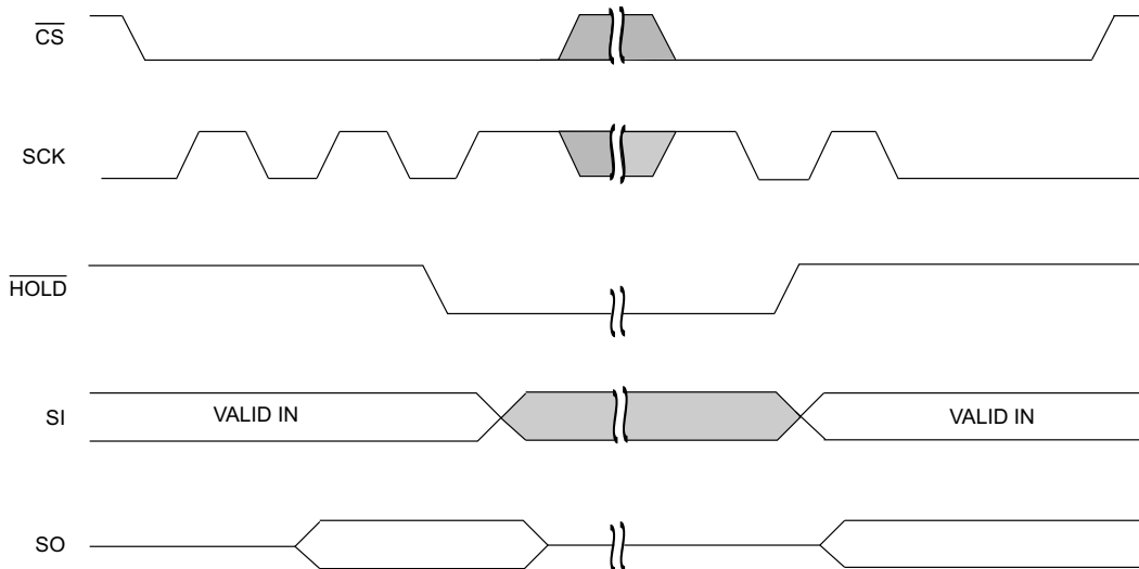
Figure 12. HOLD Operation [2]
