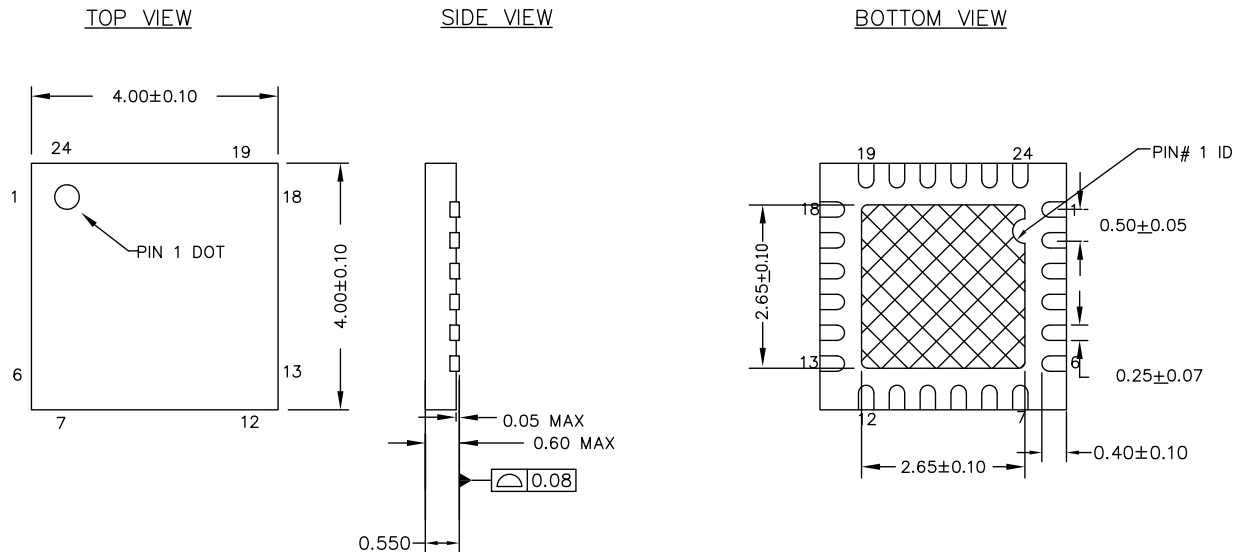
Figure 10. 24-pin QFN ( 4 \times 4 \times 0.55 mm) LQ24A ( 2.65 \times 2.65 E-Pad (Sawn)) Package Outline, 001-13937
