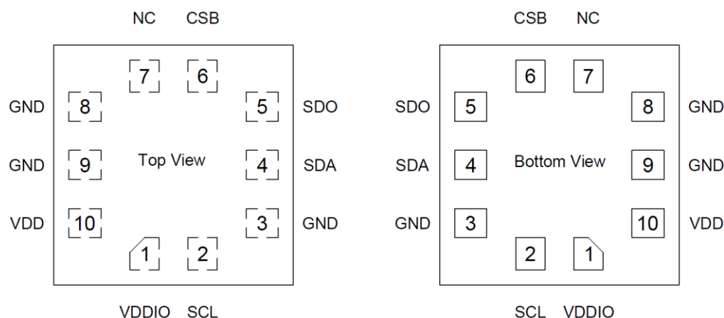
Figure 3: Layout pin configuration SPL07-003
