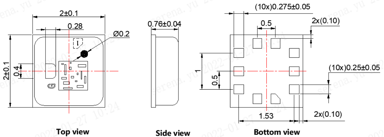
Figure 4: Top view and bottom view of SPL07-003
