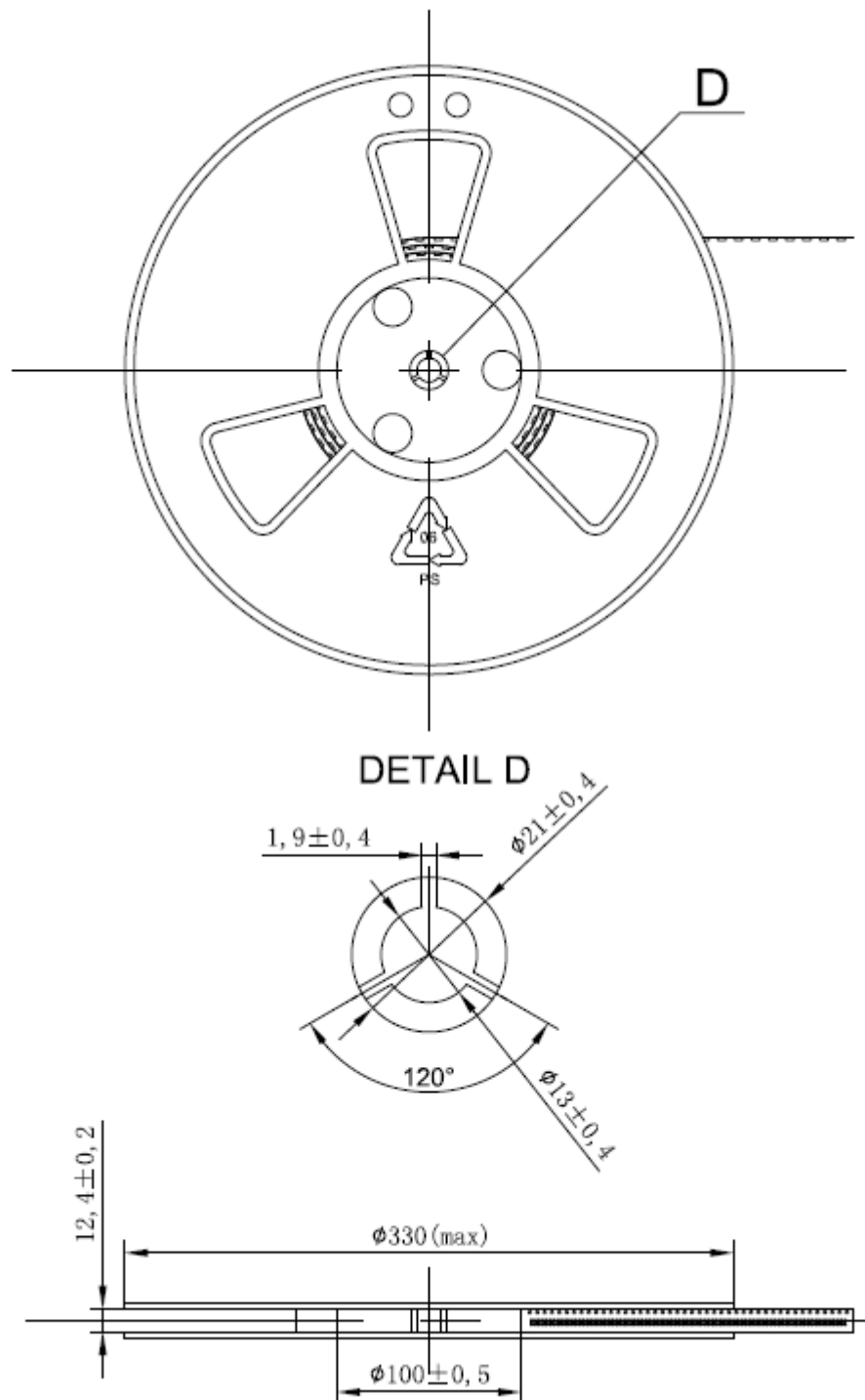
Figure 6: Carrier Tape (2)
