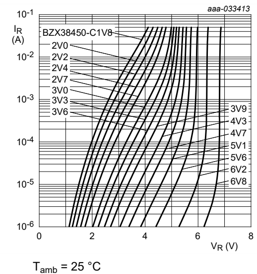
Fig. 6. Reverse current as a function of reverse voltage; typical values (BZX38450-C1V8 to BZX38450-C6V8)
