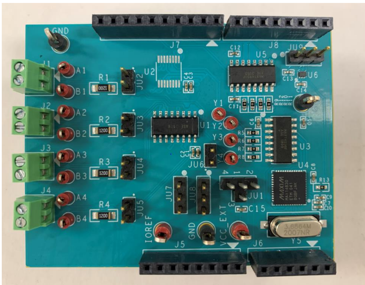
Figure 1. MAX33076E Shield
