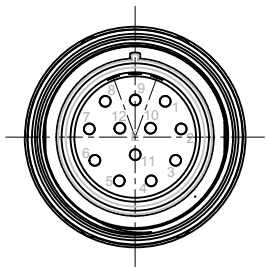
E type, Normal Key (E型, 0转位角)
