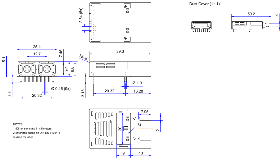
Figure 7: 1 × 9 SC Package Outline Drawings (Dimensions in mm)
