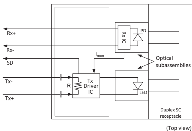
Figure 2: Block Diagram 1 x 9 SC Transceiver
