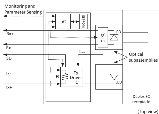
Figure 4: Block Diagram 2 x 9 SC Transceiver
