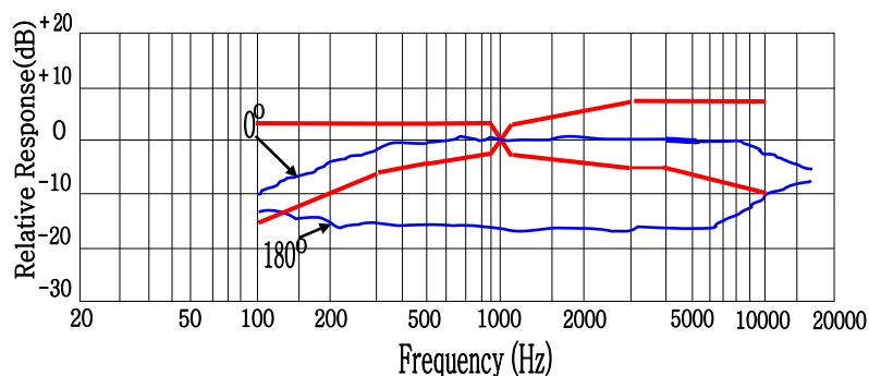
Frequency Response
