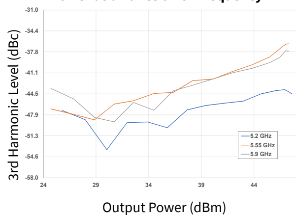
Figure 31. 3rd Harmonic vs Output Power as a Function of Frequency
