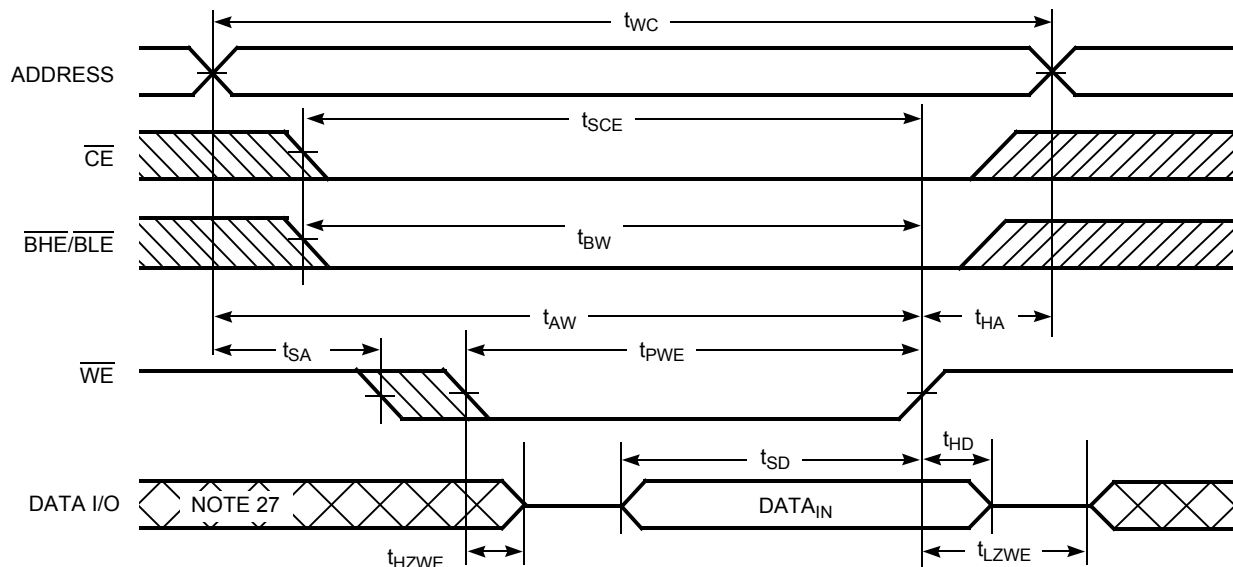
Figure 9. Write Cycle No. 4 ( \overline{\text{BHE/BL E}} Controlled, \overline{\text{OE}} LOW) [26]
