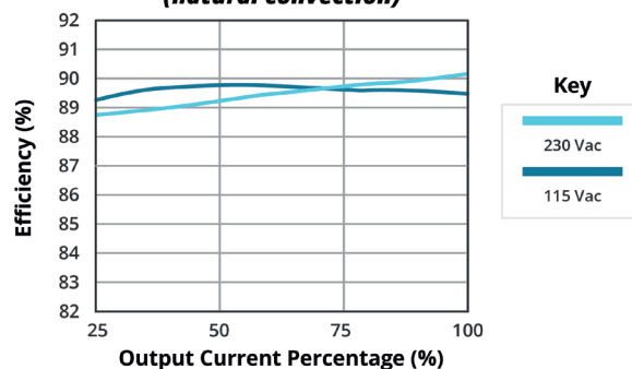
EFFICIENCY VS OUTPUT LOAD VOF-70B-24 (natural convection)
