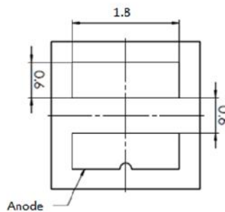
Bottom side (view through topside)
