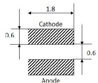
PCB Solder pad recommendation
