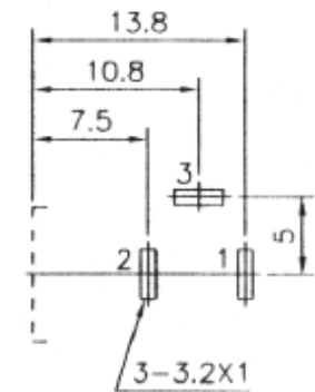
Hole Layout Bottom View
