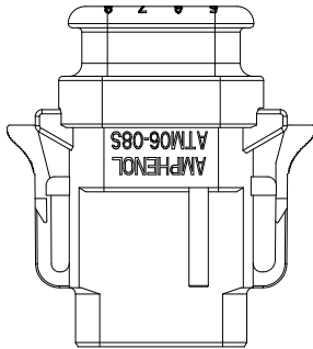
P/N ATM06-08SA-SR1GY KEY-A CONFIGURATION STANDARD COLOR: GREY
