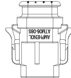
P/N ATM06-08SD-SR1BN KEY-D CONFIGURATION STANDARD COLOR: BROWN
