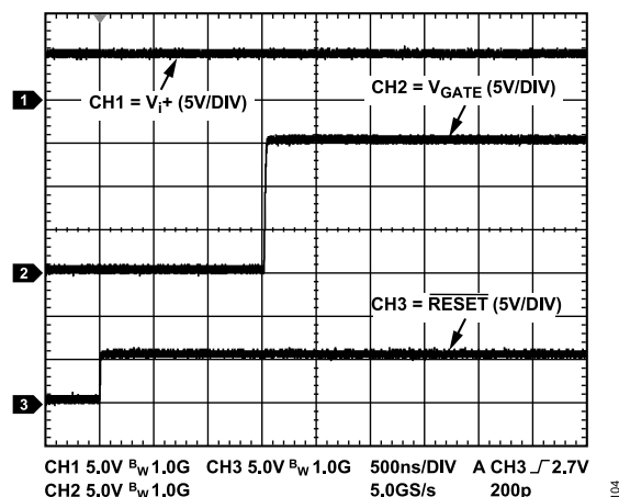
Figure 8. Typical RESET to Output Valid
