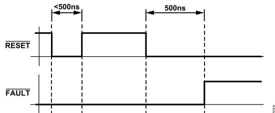
Figure 19. Timing
