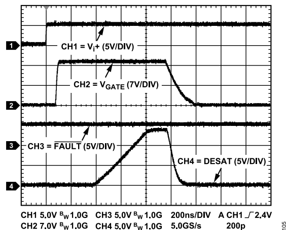
Figure 9. Example Desaturation Event and Reporting, B Grade
