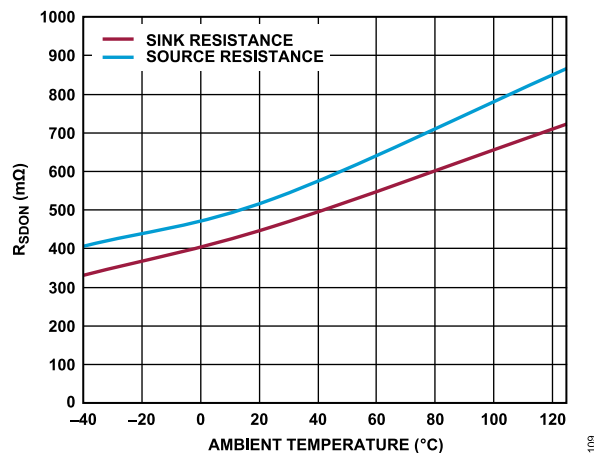
Figure 13. Output Resistance ( R_{DS(on)} ) vs. Ambient Temperature, V_{DD2} = 15\text{ V} , 250 mA Test
