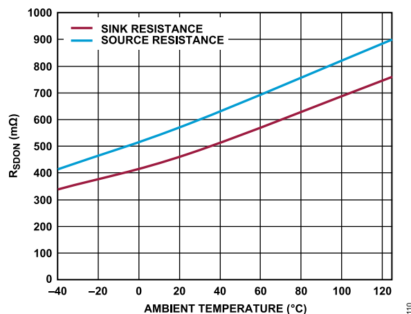
Figure 14. R_{DS(on)} vs. Ambient Temperature, V_{DD2} = 15\text{ V} , 1 A Test
