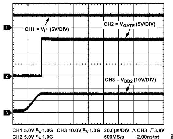
Figure 7. Typical V_{DD2} Startup to Output Valid
