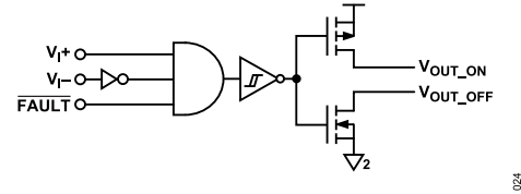
Figure 20. V_{I+} and V_{I-} Block Diagram
