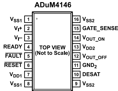
Figure 3. Pin Configuration
