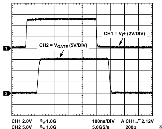
Figure 5. Typical Input to Output Waveform, 2 nF Load, 3.6 \Omega Series Gate Resistor, V_{DD1} = 5 V, V_{DD2} = 15 V, V_{SS2} = 0 V
