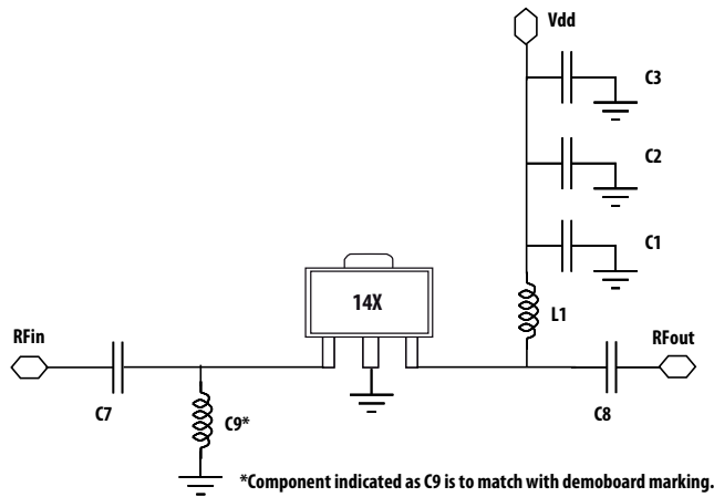
Figure 25. Circuit diagram
