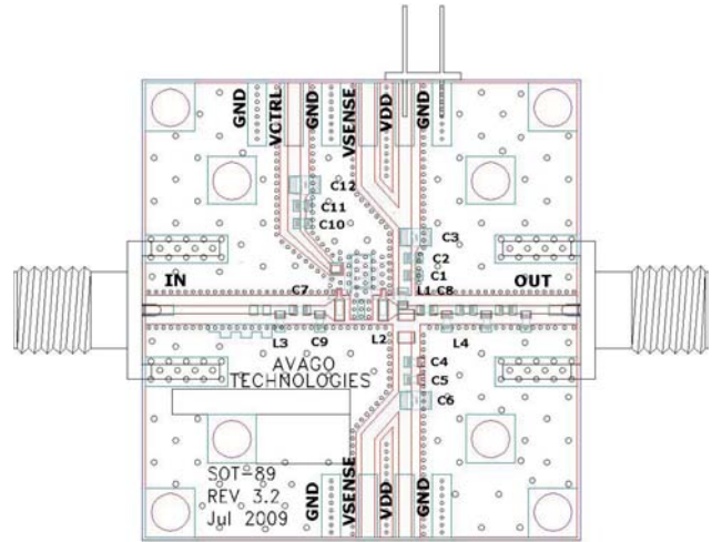
Figure 26. Demoboard
