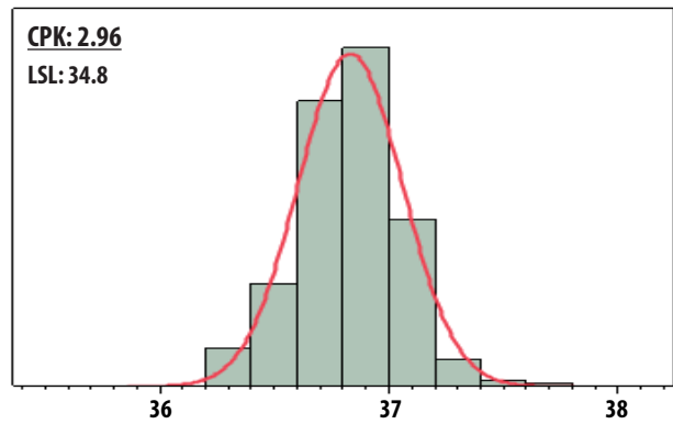
Figure 5. OIP3 @ 1900 MHz, Vd = 5 V
