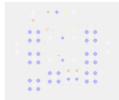
Figure 7. EVAL-ADG7421FEBZ Layer 2
