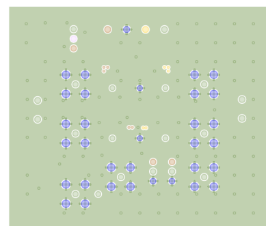
Figure 8. EVAL-ADG7421FEBZ Layer 3
