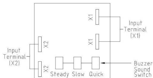
Buzzer unit bottom view:
