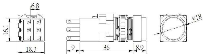
M6L-A (Round)
