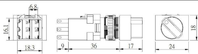
M6S-C (Rectangle)
