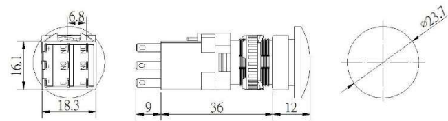
M6P-D (mushroom)
