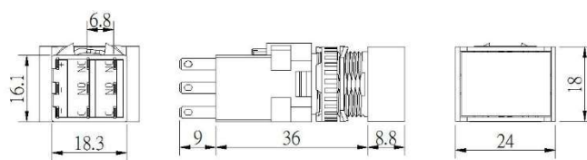
M6L-C (Rectangle)
