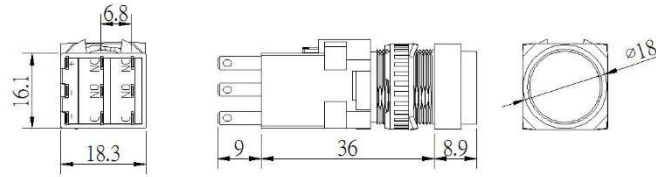
M6P-A (Round)
