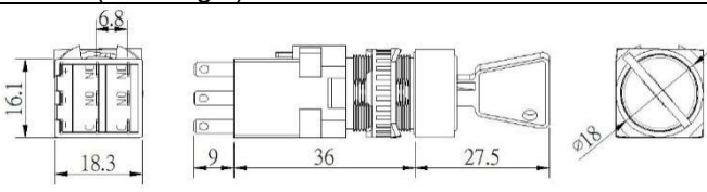
M6K-A (Round)
