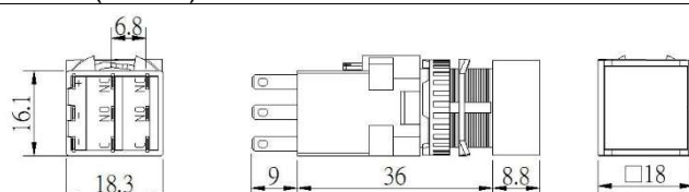
M6P-B (Square)
