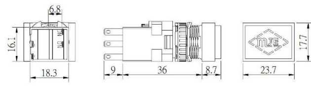
Buzzer M6Z
