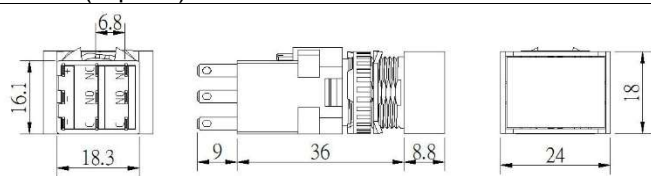
M6P-C (Rectangle)
