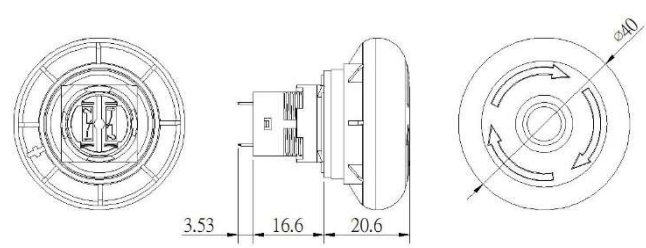
E-Stop M6E-40mm
