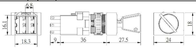
M6K-C (Rectangle)
