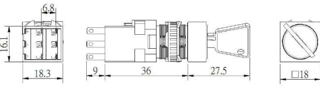
M6K-B (Square)
