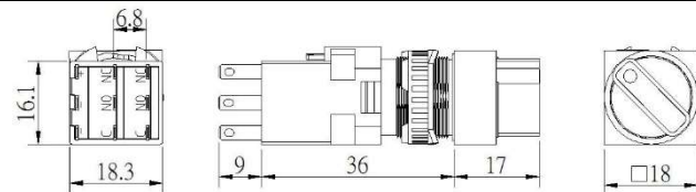
M6S-B (Square)
