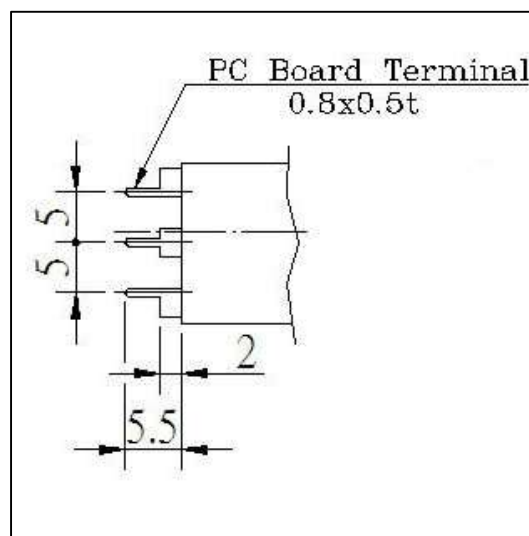
PCB Pin terminal
