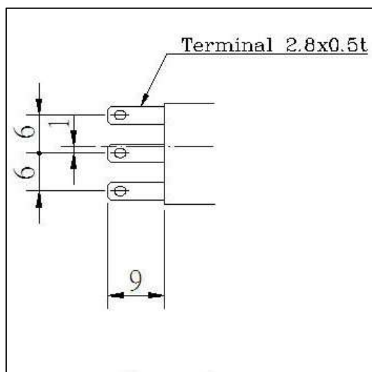
Solder, quick connect #110 terminal
