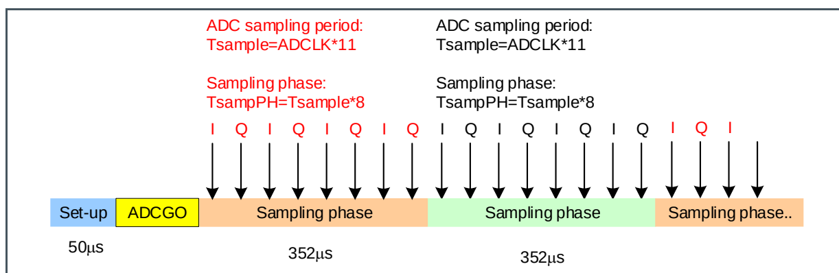
Figure 19: Measuring Cycle
