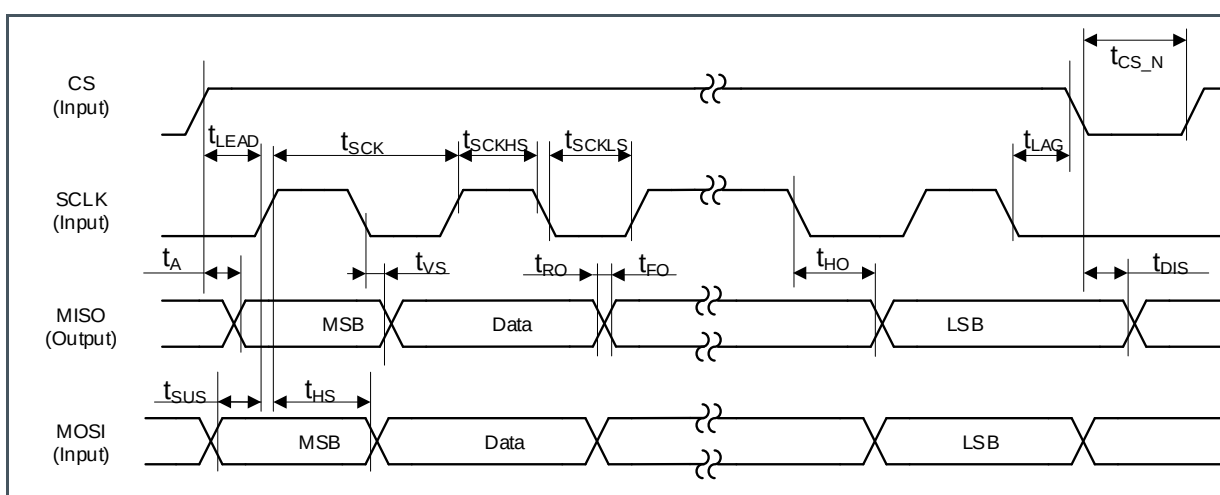
Figure 14: Timing Diagram
