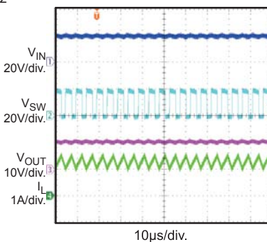
Buck-Boost Steady State
