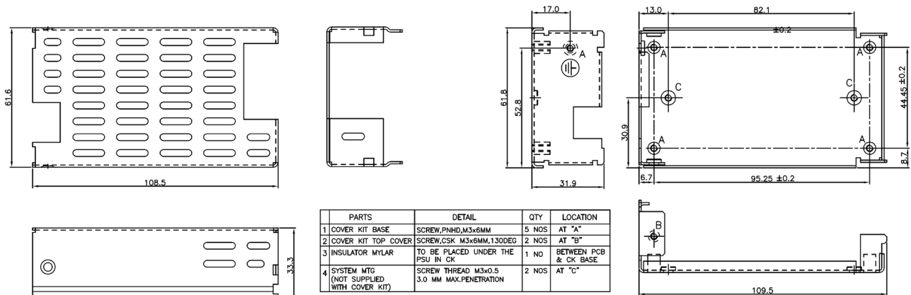
WLP225-CK. MECHANICAL OUTLINE DIMENSIONS.
