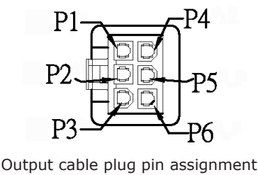
Output cable plug pin assignment
