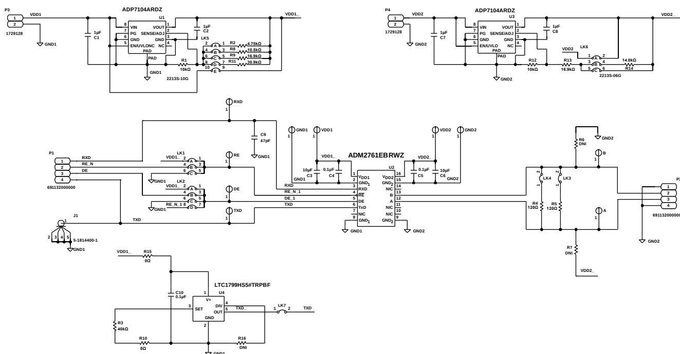
Figure 3. EVAL-ADM2761EEBZ Schematic
