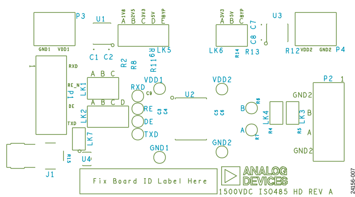
Figure 6. EVAL-ADM2761EEBZ, Silkscreen
