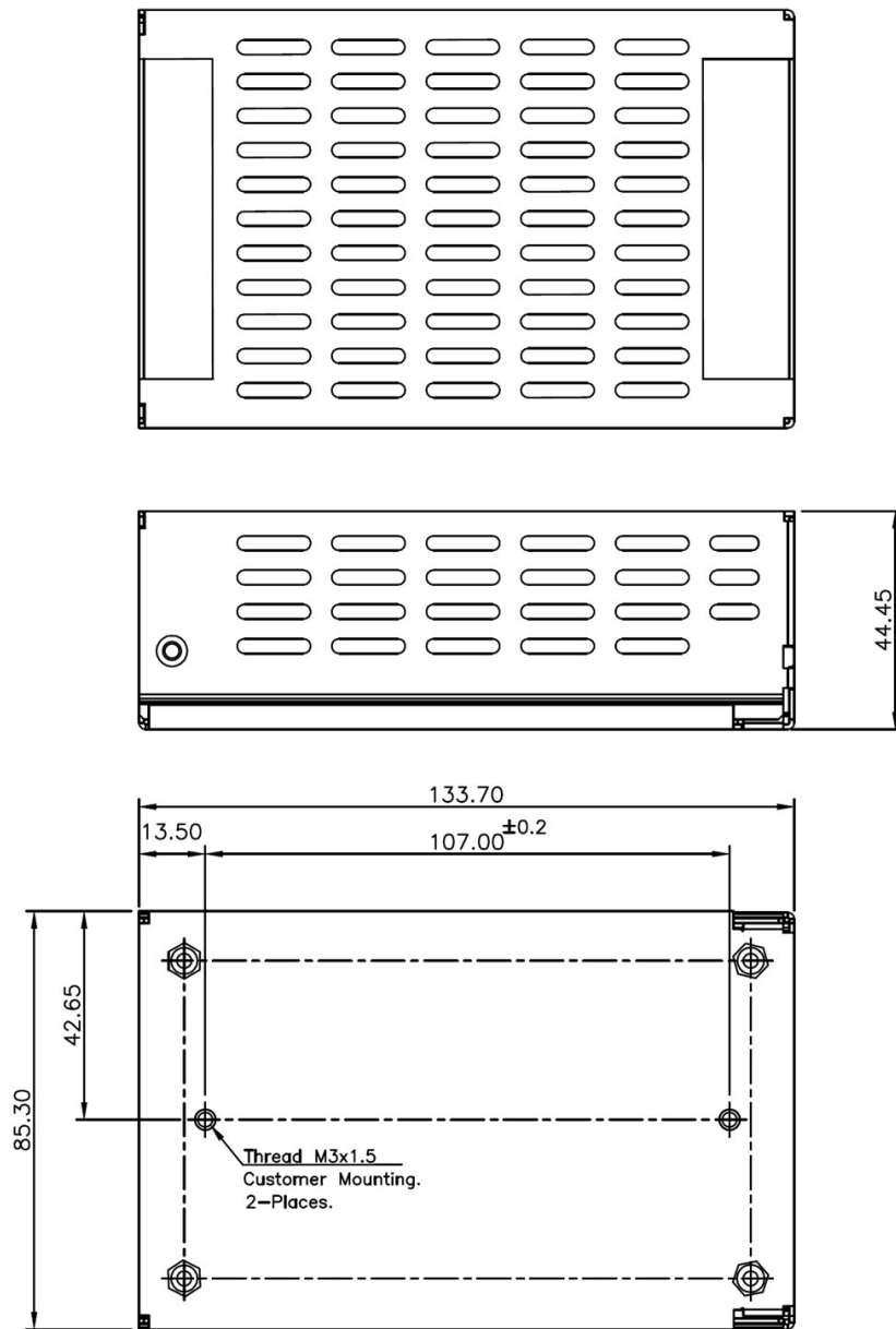
WLT200 WITH COVER KIT
