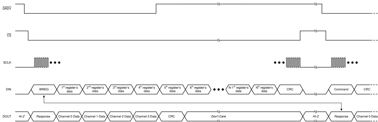
Figure 8-21. Writing Registers
